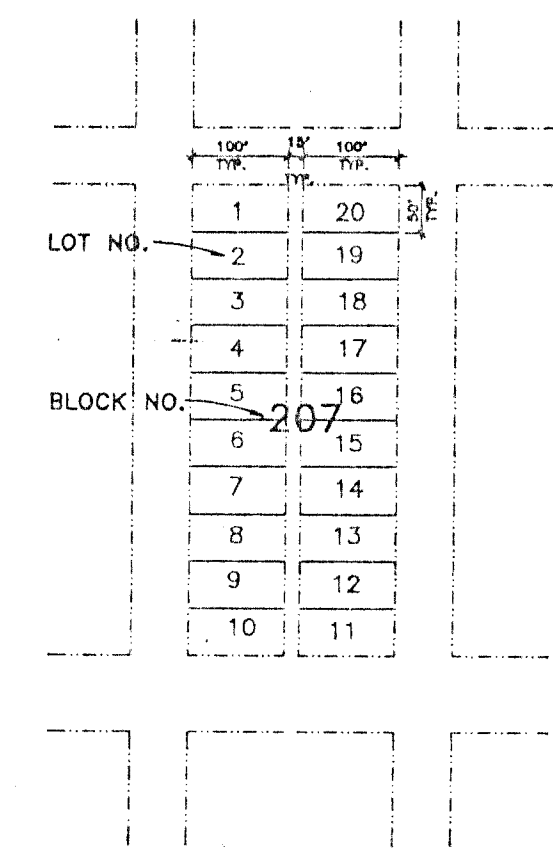
TYPICAL BLOCK (WITH DIMENSIONS)
